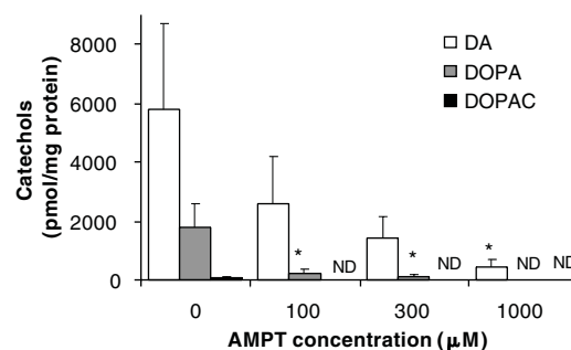
FIG. 5. Effect of AMPT on catechol levels. PC12 cells were treated with 0–1,000 \mu M AMPT, a TH inhibitor, for 72 h during differentiation. DA, DOPAC, and DOPA levels were measured using HPLC with electrochemical detection. Data are expressed as means \pm SEM ( n = 4 ). *Statistically significant from control, p < 0.05 .
