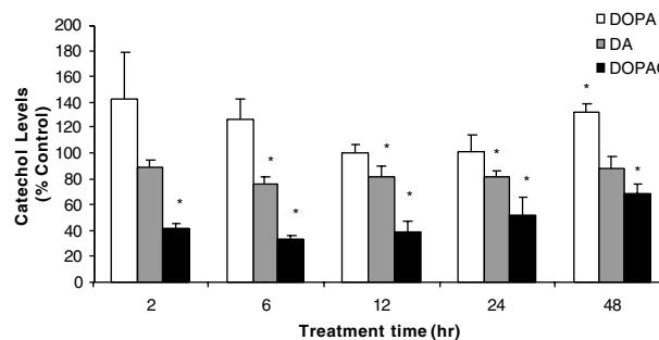
FIG. 3. Catechol levels following rotenone exposure. Differentiated PC12 cells were treated with 1 \mu\text{M} rotenone for 2–48 h. DA, DOPAC, and DOPA levels were determined using HPLC with electrochemical detection. Average control DA levels were 2.0 \pm 0.2 nmol/mg of protein. Average control DOPAC levels were 48 \pm 4.9 pmol/mg of protein. Average control DOPA levels were 511 \pm 51 pmol/mg of protein. Data are expressed as mean % control \pm SEM ( n = 4-5 ). *Statistically significant from control, p < 0.05 .
