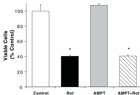
FIG. 6. PC12 cell viability following DA depletion and rotenone exposure. PC12 cells were treated with 1 mM AMPT or control medium for 72 h, followed by 1 \mu M rotenone or vehicle for 48 h. Cell viability was then determined using trypan blue exclusion. Data are expressed as mean % control \pm SEM ( n = 4 ). *Statistically significant from control, p < 0.05 .
