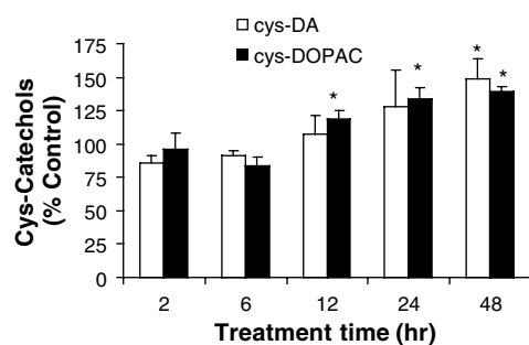
FIG. 4. Protein cysteinyl-catechol levels following rotenone exposure. Differentiated PC12 cells were treated with 1 \mu M rotenone for 2–48 h. Protein cysteinyl-DA and protein cysteinyl-DOPAC levels were determined using HPLC with electrochemical detection. Data are expressed as mean % control \pm SEM ( n = 4 –6). *Statistically significant from control, p < 0.05 .
